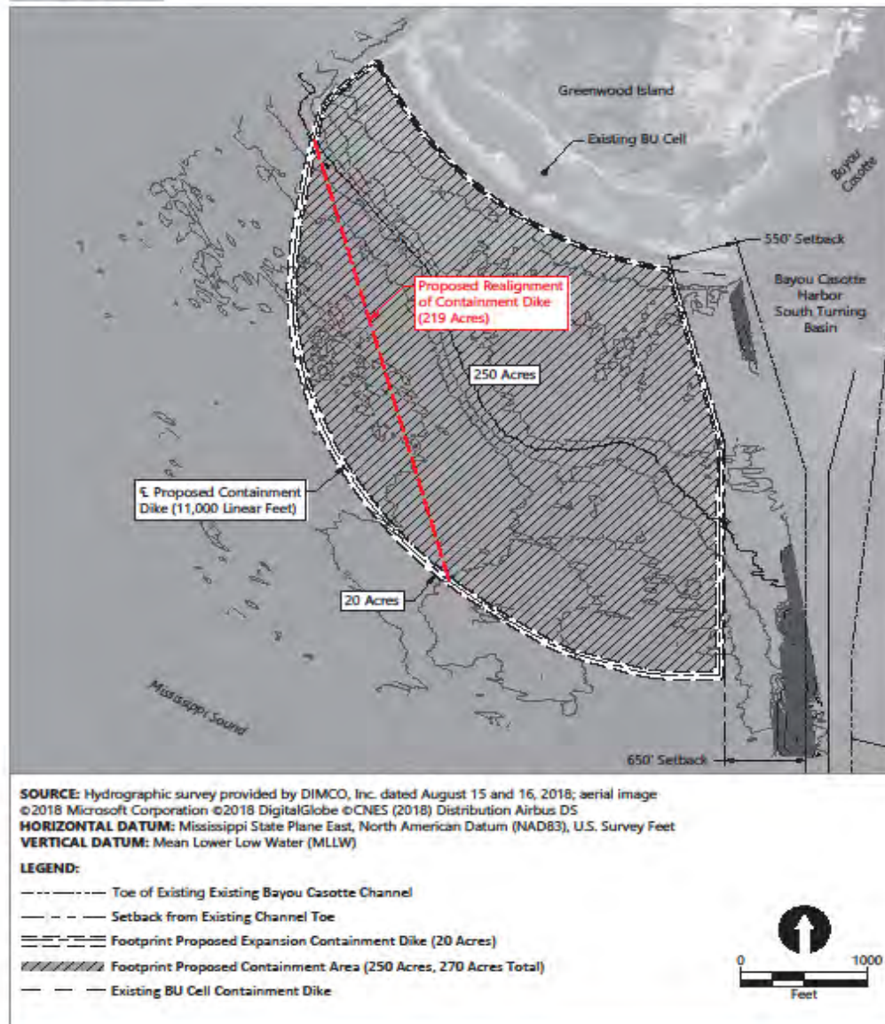
Figure 2 Proposed Containment Dike Alignment Greenwood Island Beneficial Use Expansion Permit Mississippi Department of Environmental Quality
